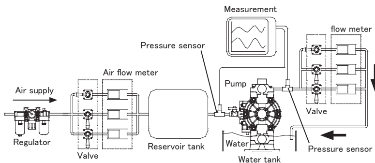
Measurement equipment and piping layout diagram
